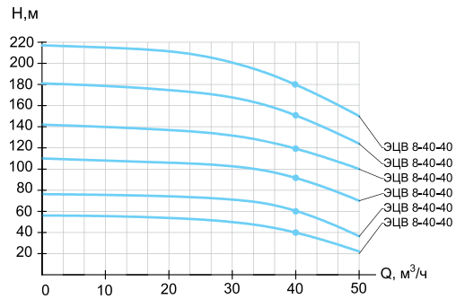
ЭЦВ 8-40
