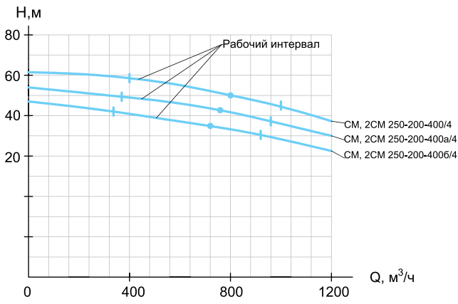
CM, 2CM 250-200-400/4
