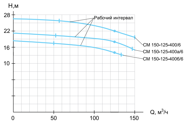
CM 150-125-400/6
