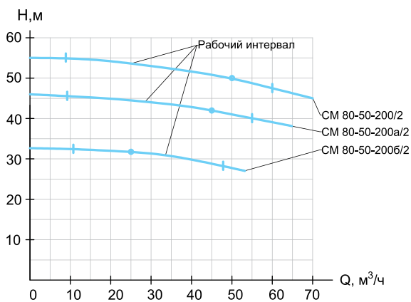
CM 80-50-200/2
