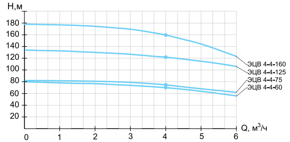
ЭЦВ 4-4
