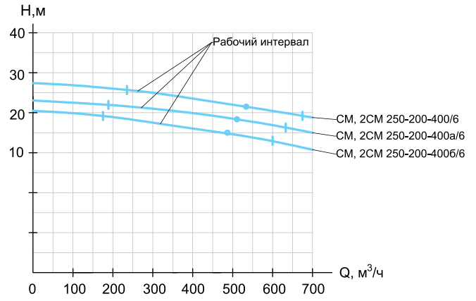
CM, 2CM 250-200-400/6
