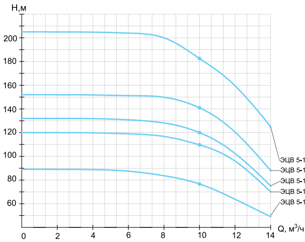
ЭЦВ 5-10
